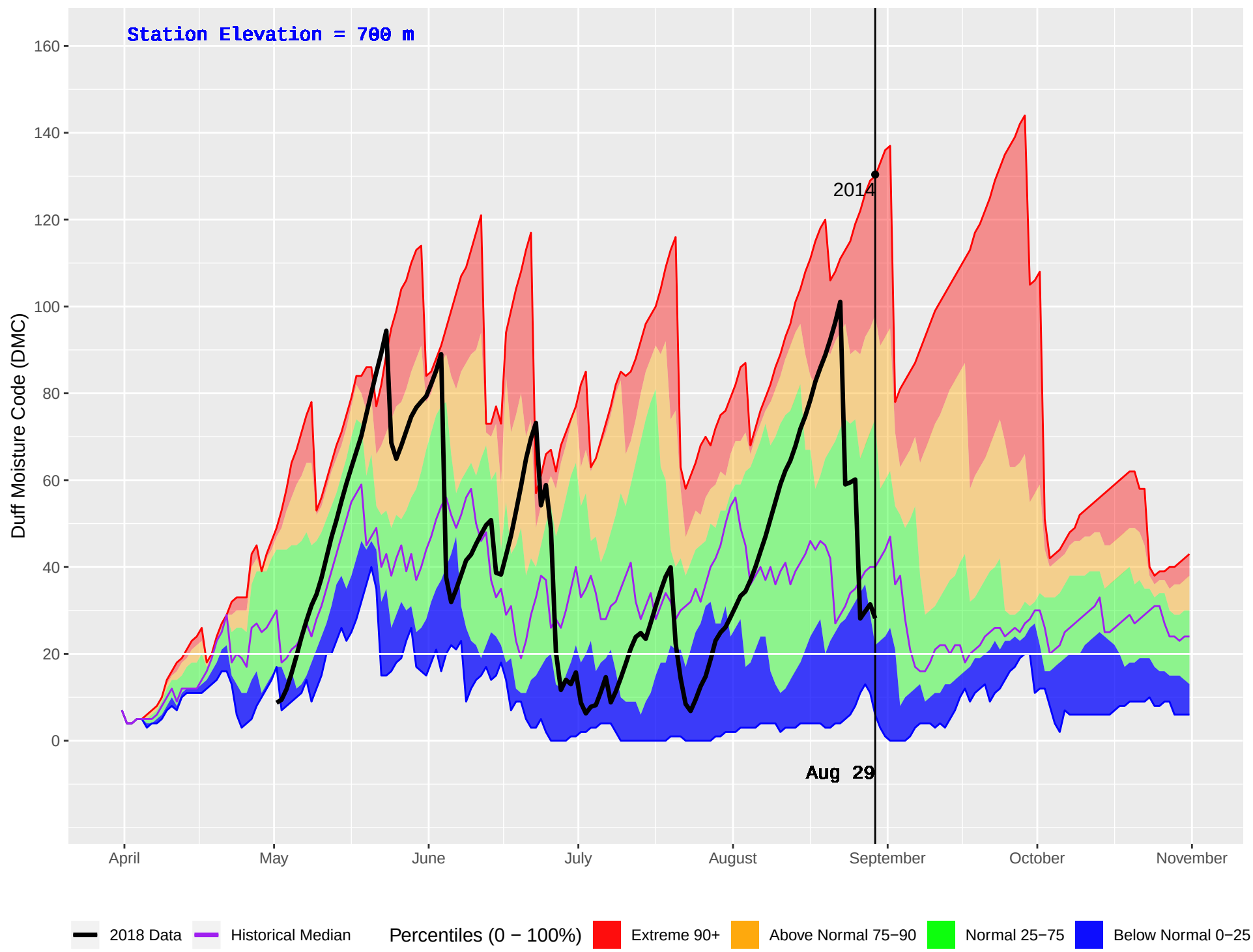
OSBORN (1045) : Historical (2009–2016) and Current (2018) Daily Duff Moisture Code (DMC)
